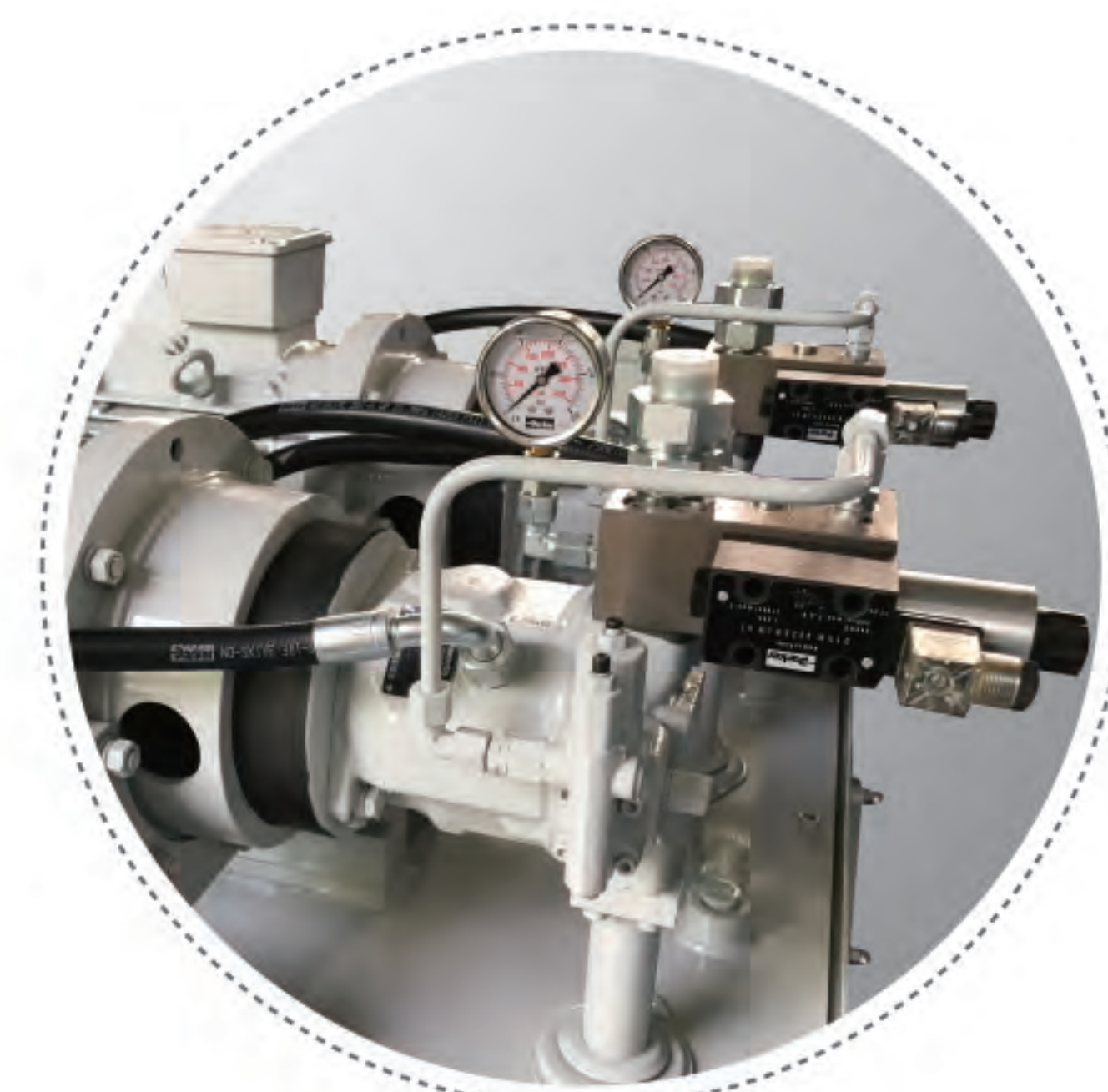
● 泄压及安全阀模块 Module of decompression and safety valves
