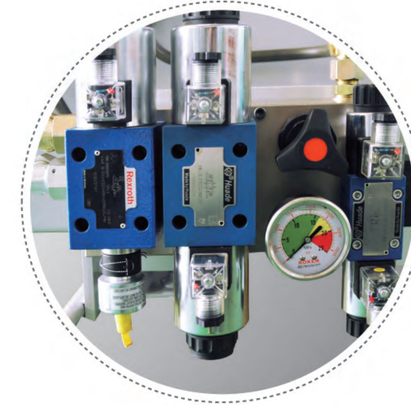
• 系统局部特写 Partial features of the system
